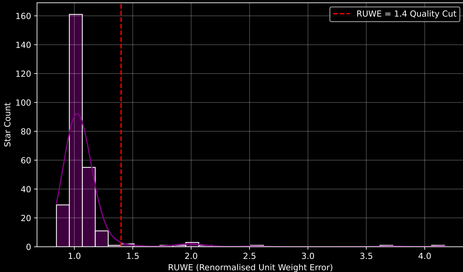
GAPOGEE DR17 Field [109+12] RUWE Distribution (n= 268)
