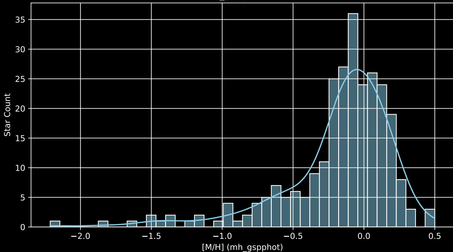
APOGEE DR17 Field: [109+12 [M/H] (mh_gspphot) (n= 266)
