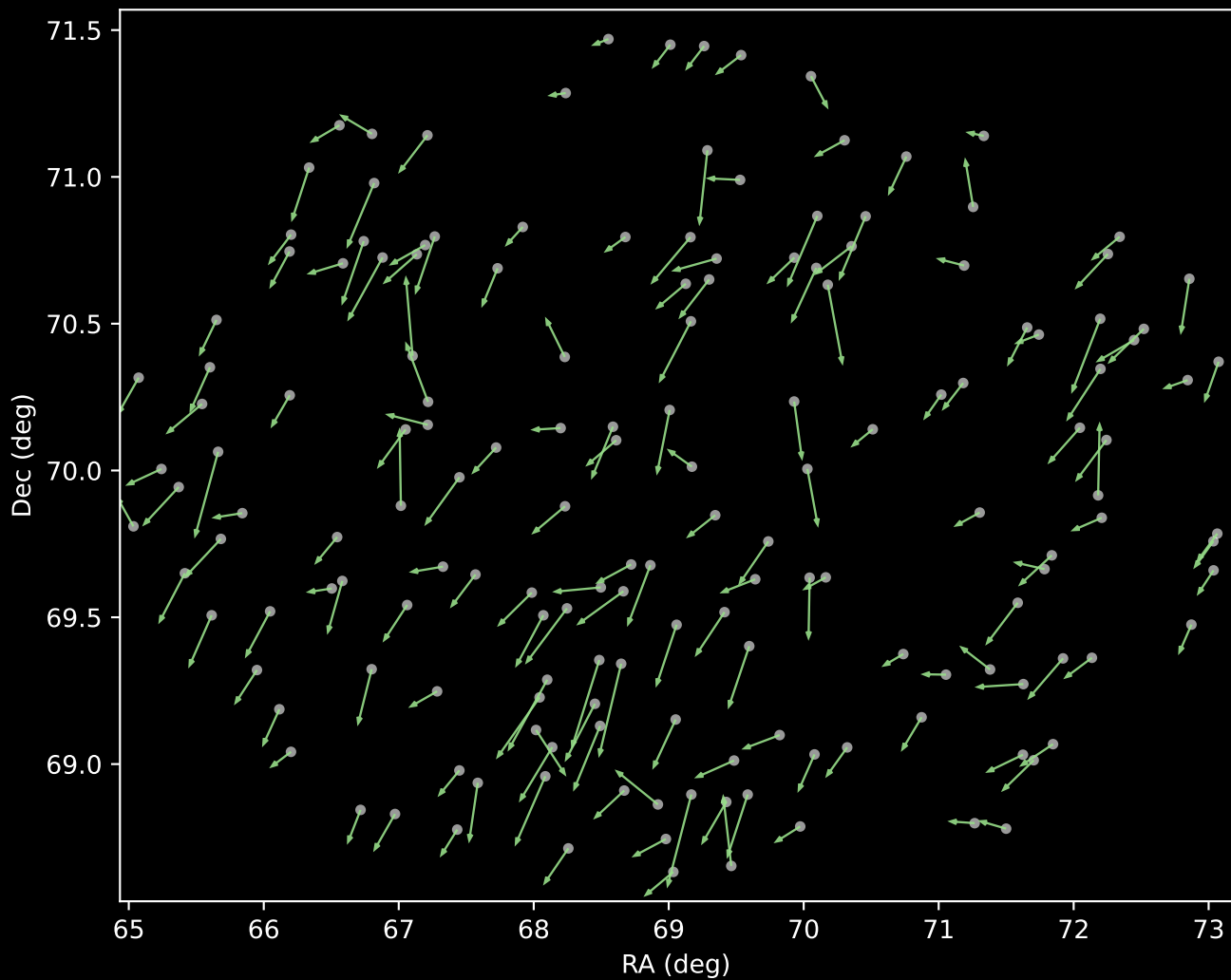
APOGEE DR17 Cluster 5 Proper Motion Vectors (n=163)
