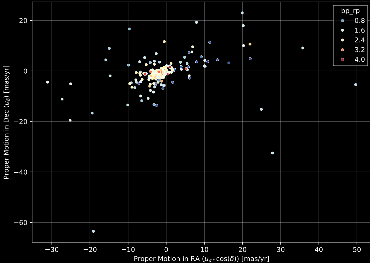
APOGEE DR17 Field: [109+12] Proper Motion Diagram (n= 268)
