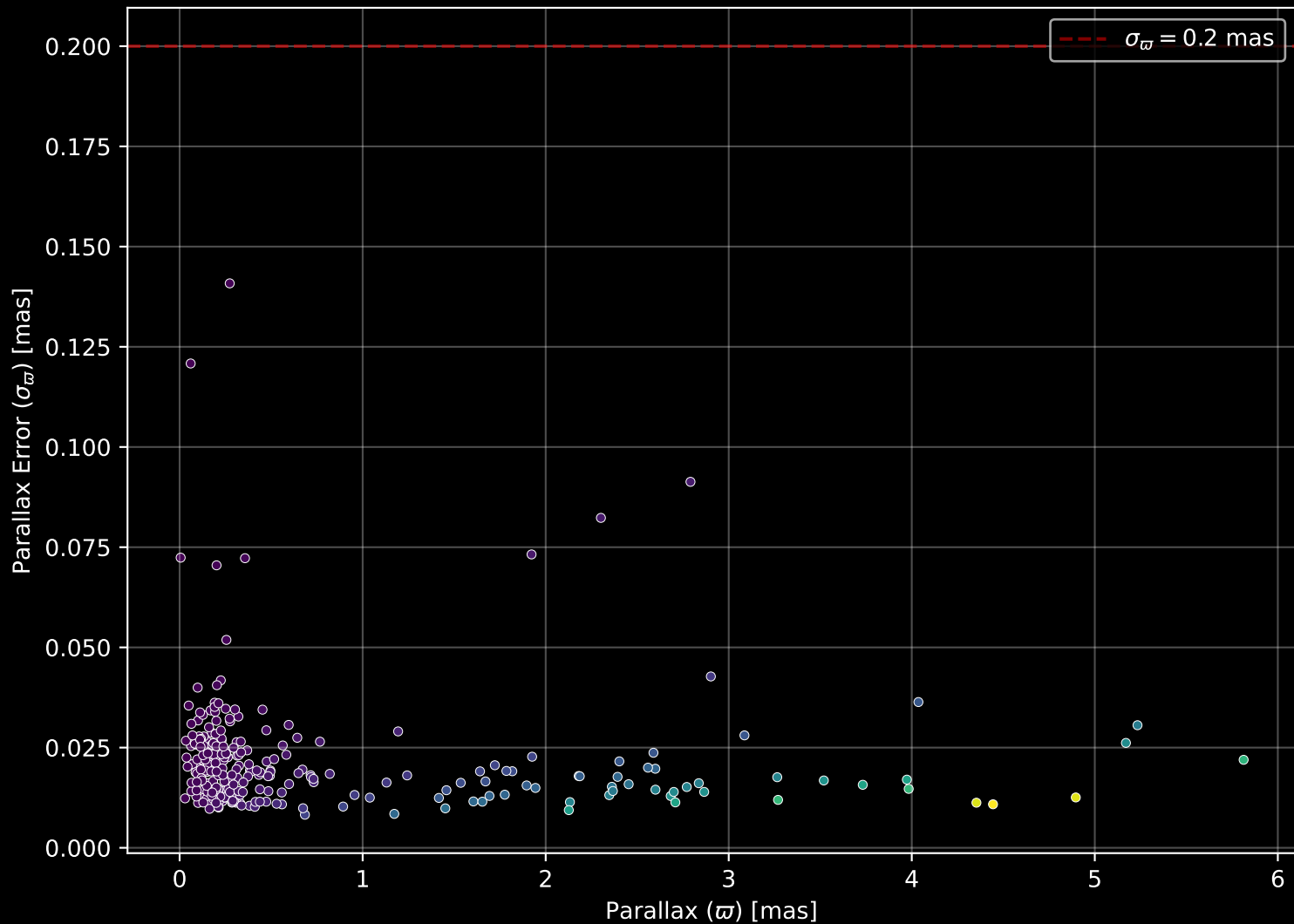
APOGEE DR17 Field: [109+12] Parallax Quality (n= 268)
